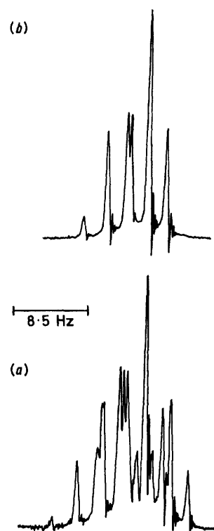
FIGURE 2 60-MHz Proton n.m.r. spectra of a mixture of \text{NMe}(\text{PCl}_2)_2 and \text{NMe}(\text{PBr}_2)_2 showing resonances due to intermediate species: (a) normal spectrum; (b) with {}^{31}\text{P} decoupling [from left to right the peaks are assigned to species (15), (14), (13), (12), (11), and (10) respectively]
