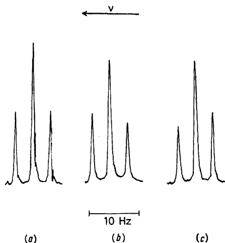
FIGURE 1 N -Methyl proton resonance of \text{NMe}[\text{P}(\text{OMe})_2]_2 at 60 MHz: (a) normal spectrum; (b) with simultaneous irradiation at [\nu(^{31}\text{P}) - {}^2J(^{31}\text{P} \cdots ^{31}\text{P})] and \gamma(^{31}\text{P})B_2/2\pi \approx 25 Hz; and (c) with simultaneous irradiation at [\nu(^{31}\text{P}) + {}^2J(^{31}\text{P} \cdots ^{31}\text{P})] and \gamma(^{31}\text{P})B_2/2\pi \approx 25 Hz
